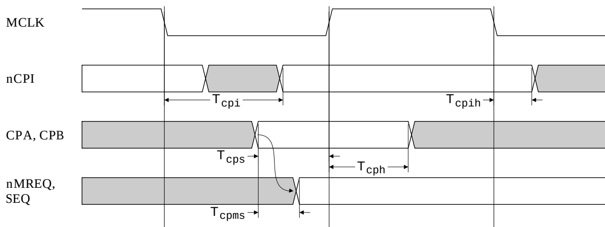
Figure 41: Coprocessor Timing
