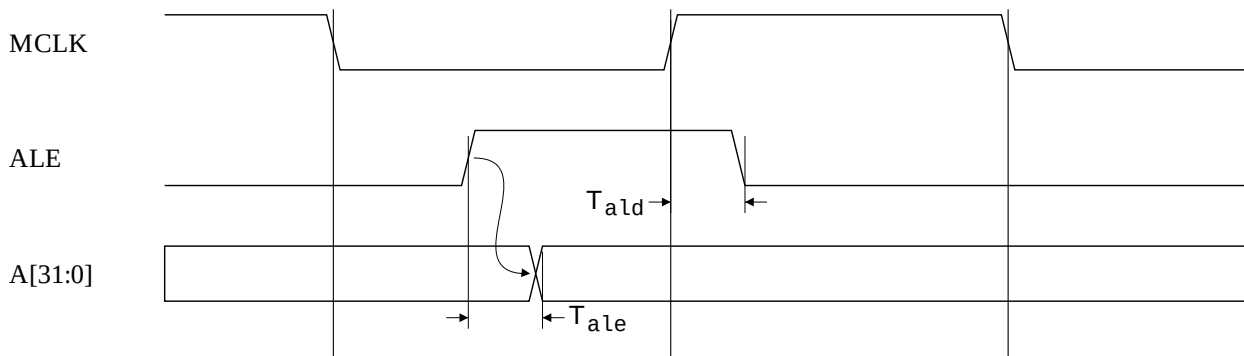
Figure 36: Address Timing
