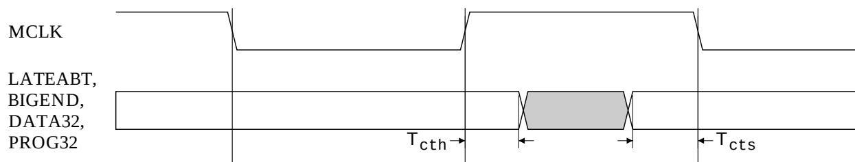
Figure 40: Configuration Pin Timing
