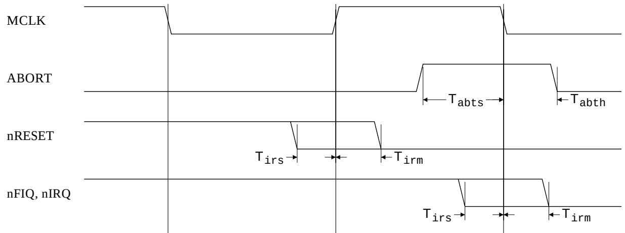
Figure 42: Exception Timing
