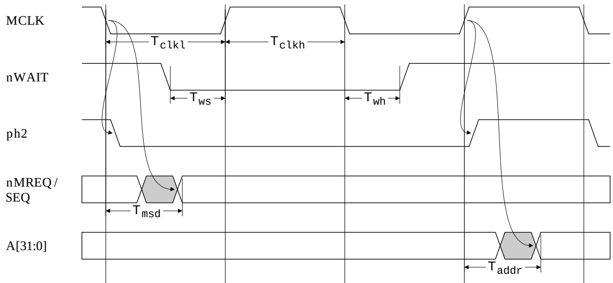
Figure 43: Clock Timing
