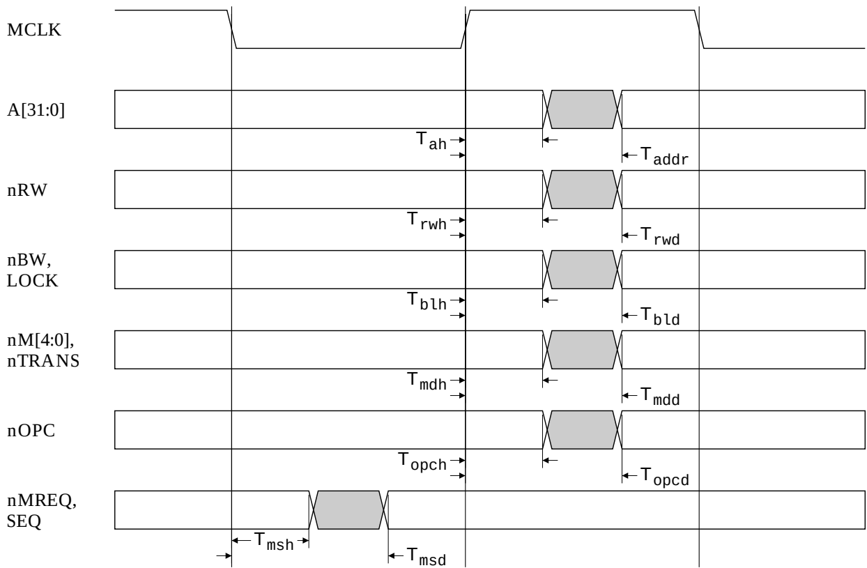
Figure 35: General Timings
